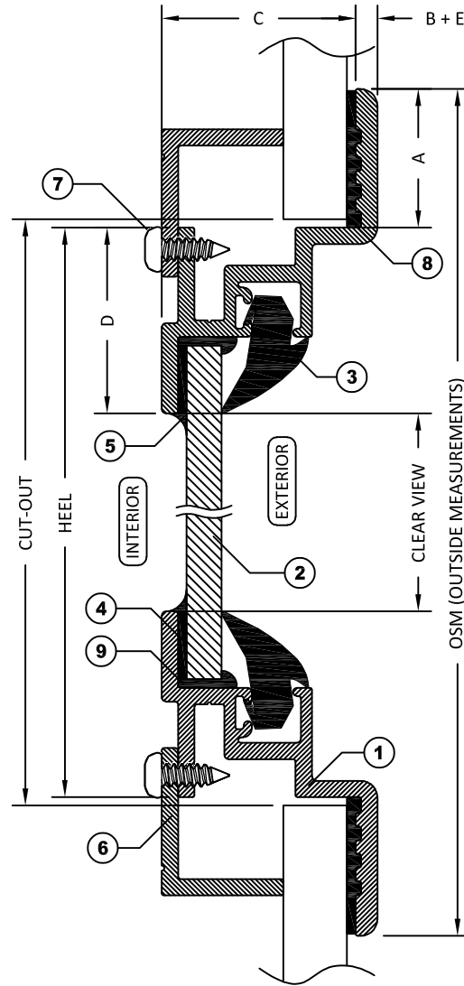
SECTION A-A WITH CLAMP IN INSTALLATION
