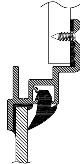
OPTIONAL BOLT-ON INSTALLATION
