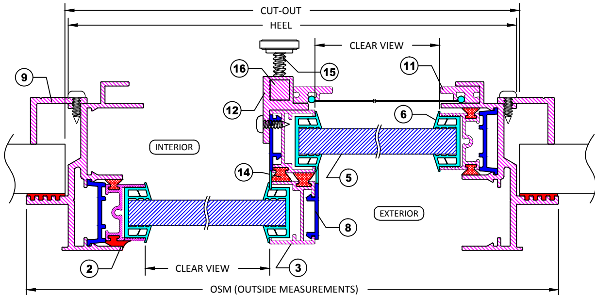
SECTION A-A WITH CLAMP IN INSTALLATION
