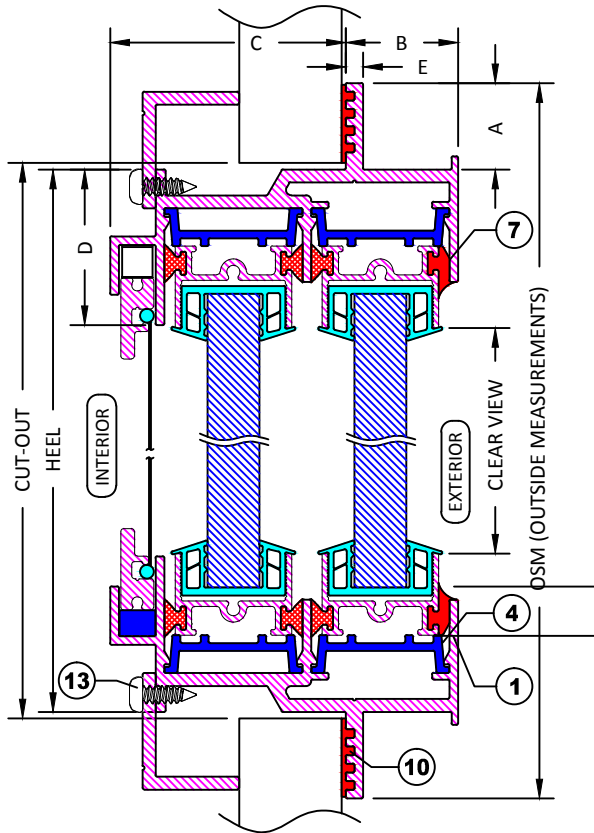
SECTION B-B WITH CLAMP IN INSTALLATION
