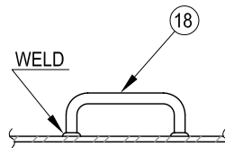
DETAIL OF GRAB HANDLE
