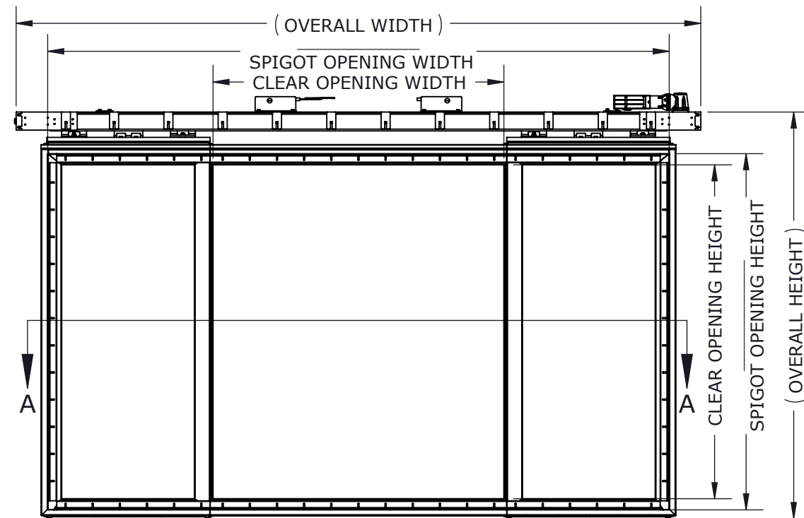
INTERIOR VIEW (OPEN)
