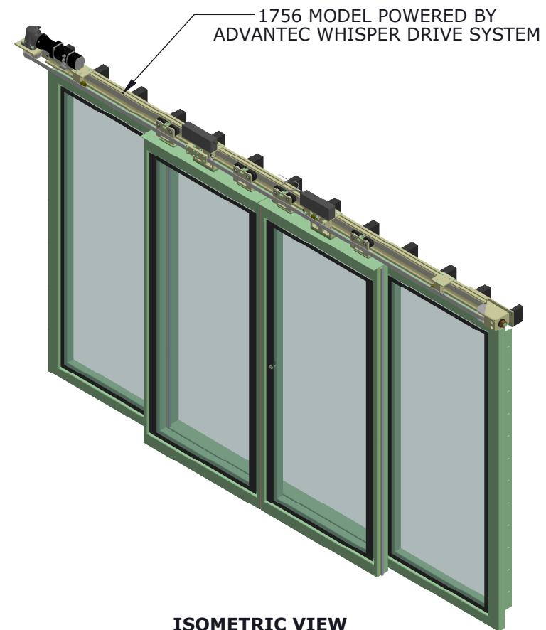
ISOMETRIC VIEW SCALE 1 : 30
