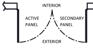
LEFT HAND OUTWARD OPENING ACTIVE
