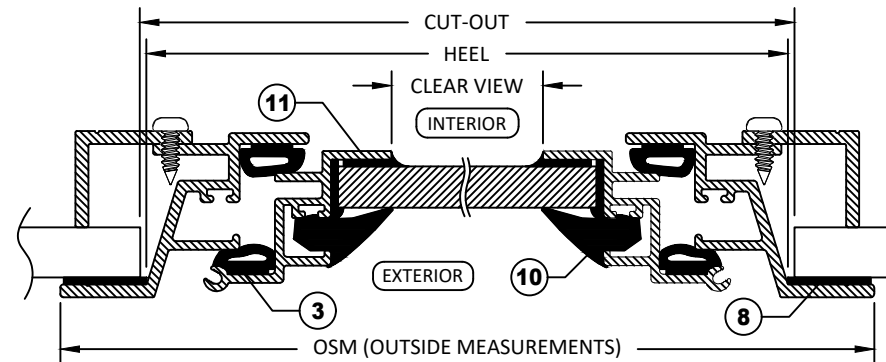
SECTION A-A WITH CLAMP IN INSTALLATION
